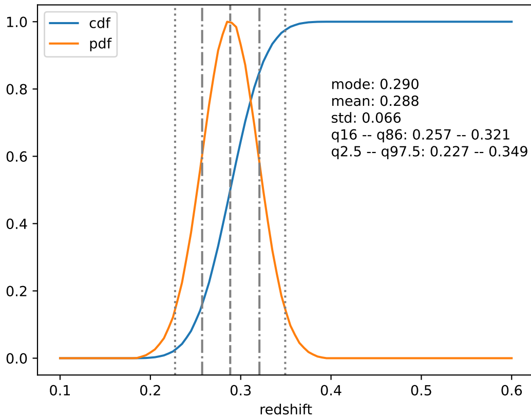
FIGURE 16: Single object p(z) estimate, showing both the PDF, and the CDF, as well as the summary statistics described in the text.
