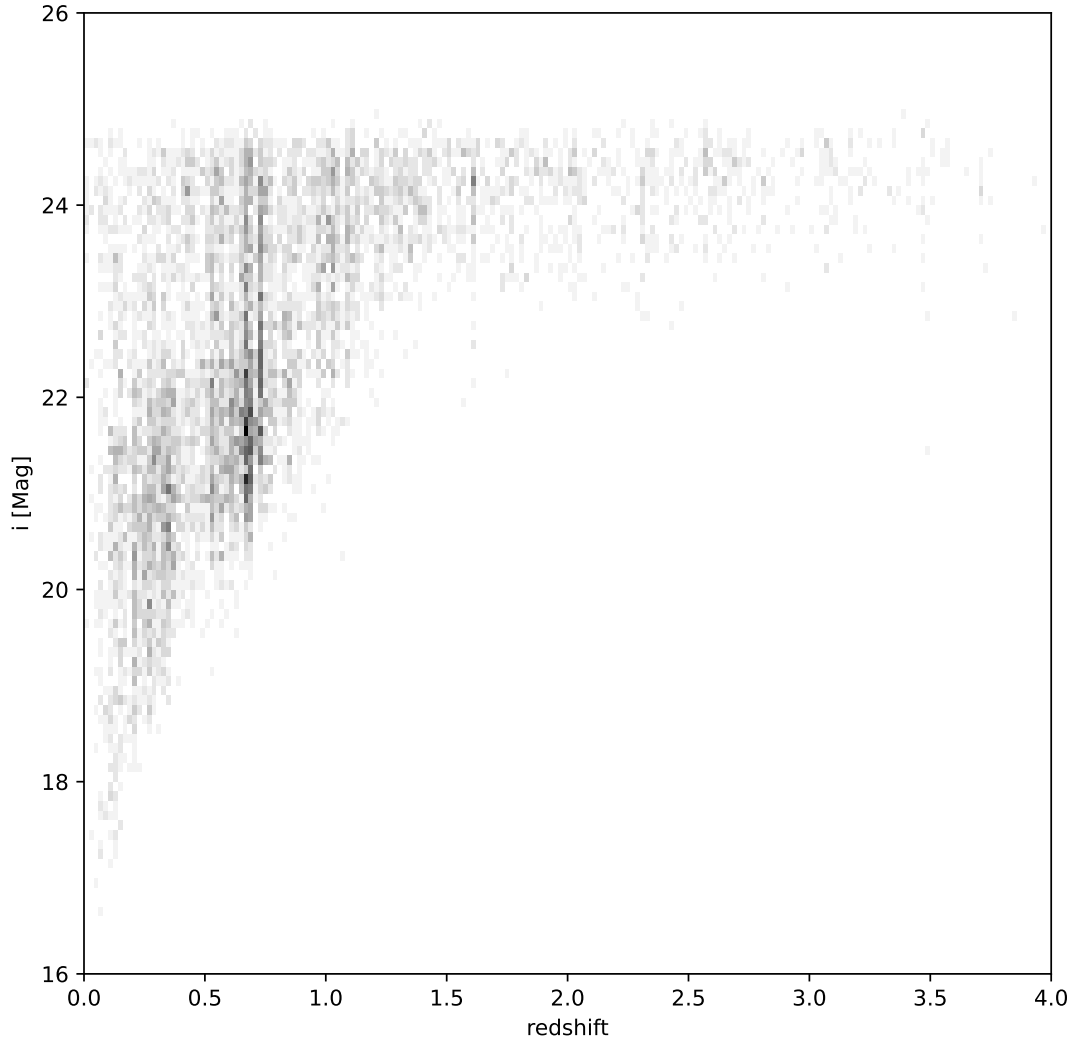
FIGURE 2: 1.0 arc-second Gaussian Aperture (Gaap) i-band magnitude versus redshift for all objects in the “test_v1” dataset.
