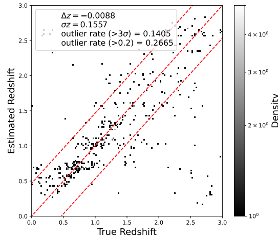
FIGURE 15: Point-estimates versus spectroscopic redshifts for all galaxies in the reserved test set with m_i > 24.0 , showing the degradation in estimation performance for faint objects.
