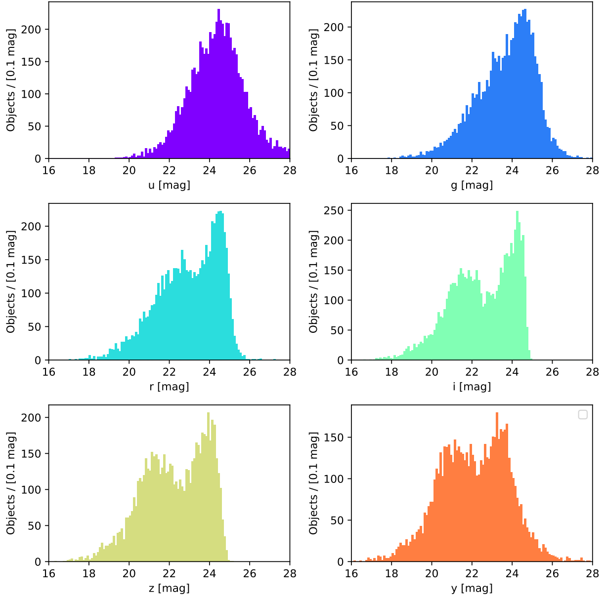
FIGURE 1: 1.0 arc-second Gaussian Aperture (Gaap) magnitudes (in AB system) of objects in each of the six Rubin filter bands in the “test_v1” dataset. These aperture magnitudes were used as the inputs for the photo- z algorithms.
